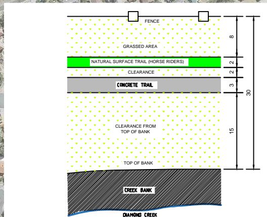
DIAMOND CREEK TO HURSTBRIDGE OFF ROAD TRAIL TYPICAL LAYOUT PLAN - (Not to scale)
